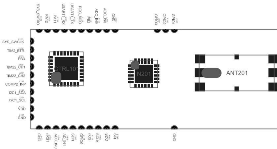
Figure 3: SIGFOX-MOD1/2-C Layout
