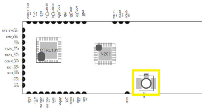
Figure 5: SIGFOX-MOD1/2-E Layout
